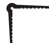
2 'D' SECTION Standard Length 3000mm Material EPDM Rubber Fixing method 10mm dia Expanding Anchor Bolts (8 No.) @ 400mm centres
