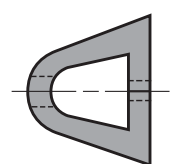
2 'D' SECTION Standard Length 3000mm Material EPDM Rubber Fixing method 10mm dia Expanding Anchor Bolts (8 No.) @ 400mm centres
