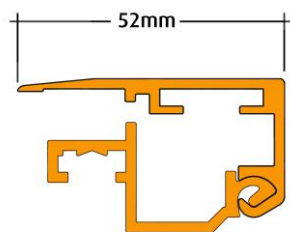
Lockable Frame
