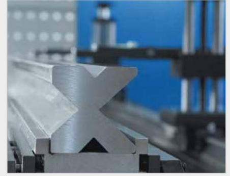
► Standard centring rail with optional, tempered and polished Multi-V die
