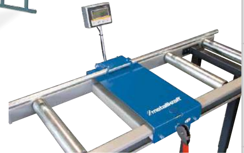
MRB LC-E with magnetic strip, length measuring device with digital display and 4x roller borne stop carriage
