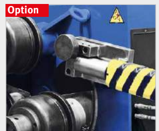
▶ Option: two lateral hydraulic guide rollers
