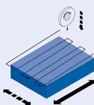
Surface grinding with feed at start point
