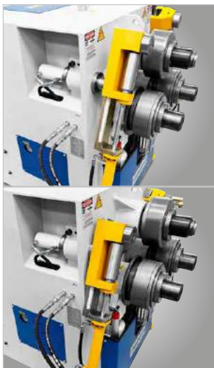
Lateral mechanical straightening rollers, continuously adjustable
