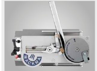
Anti-clockwise bending
