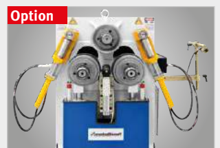
▶ Option: two lateral hydraulic guide rollers
