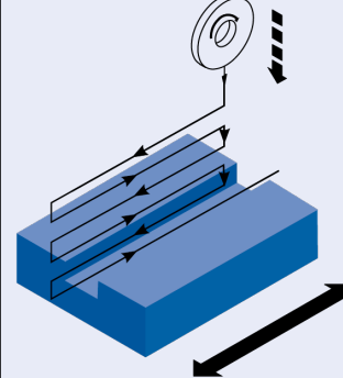
Groove grinding with feed at start point
