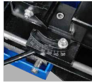
▶ Grinding angle of 30-90° adjustable based on scale
