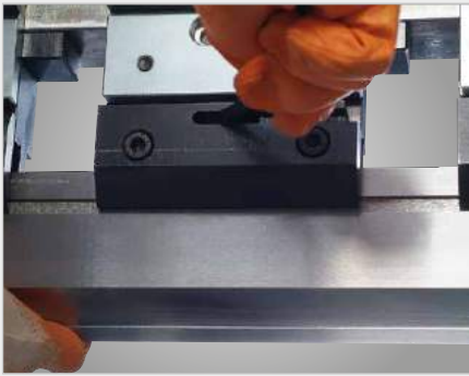
► Manual quick release clamping for fast tool changes (standard for R, S and Servo)
