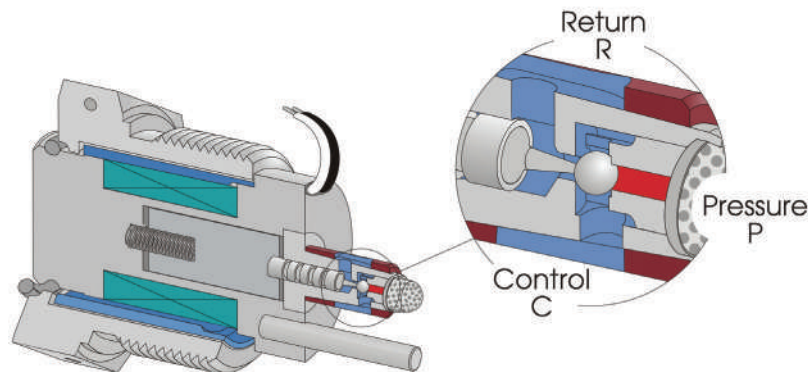
Standard 3-way, single coil, normally closed configuration
