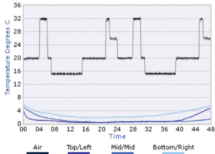
Example of a Poly Shipper Flat Pack System (PFP57) - Tested against a 48 hour summer ramp
